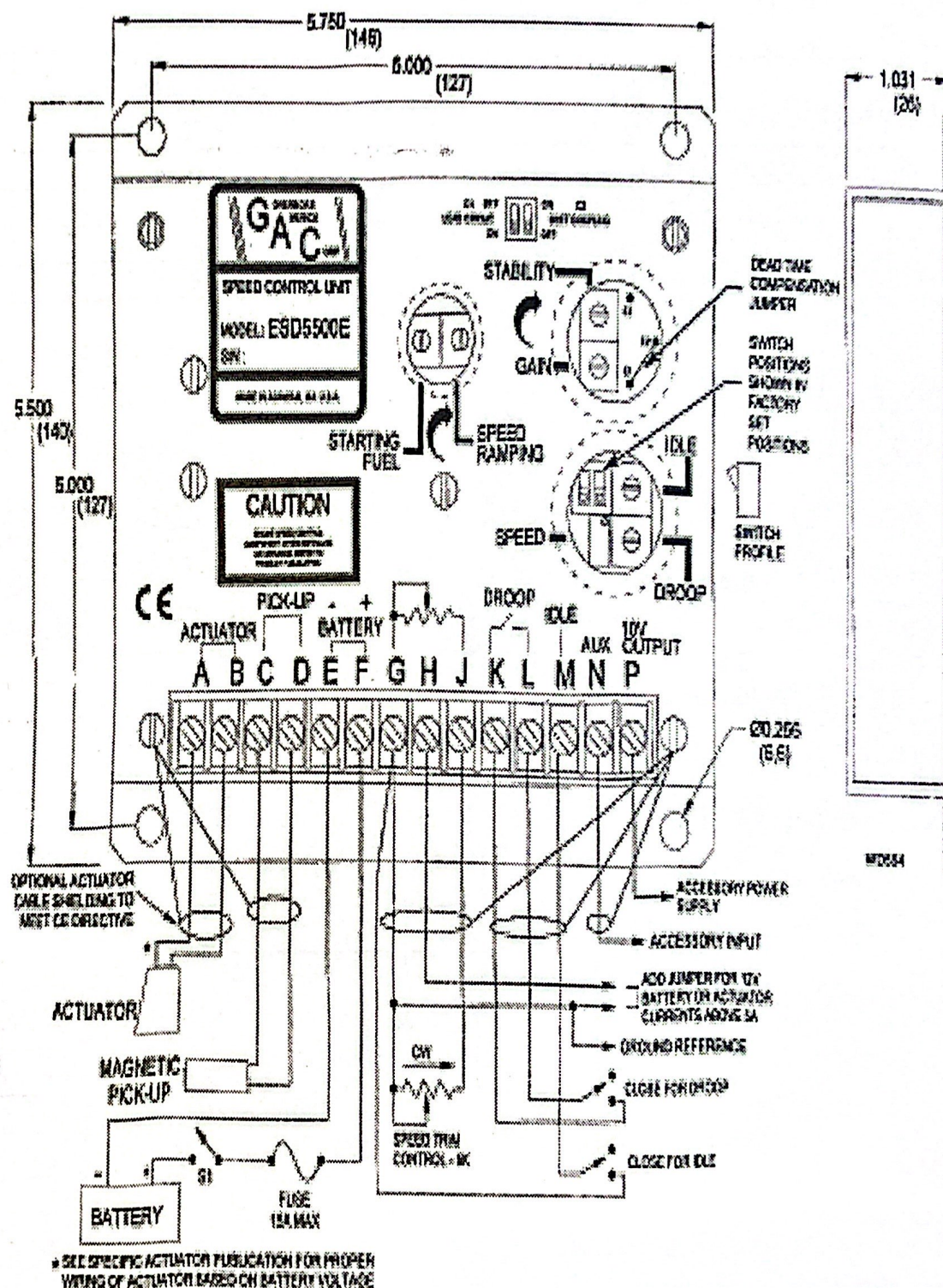
DIAGRAM 1. ESD5500E Series Wiring Diagram and Outline
